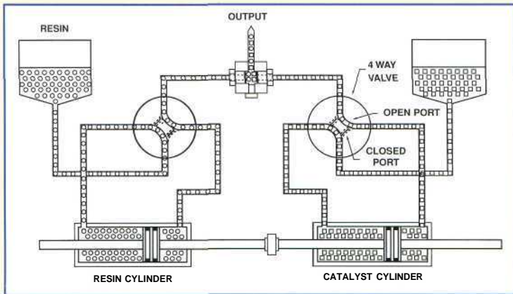
2500 DOUBLE ACTING FLOW SCHEMATIC
